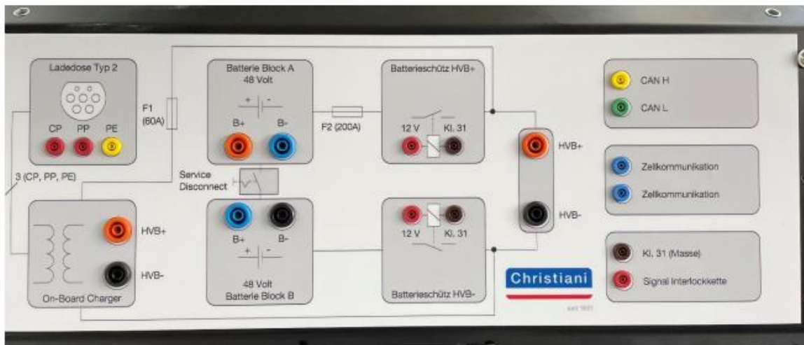
Measuring field power supply module
