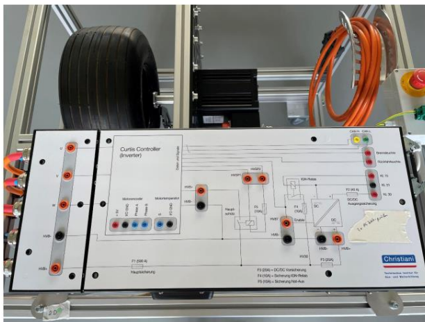
Measuring field for motor control
